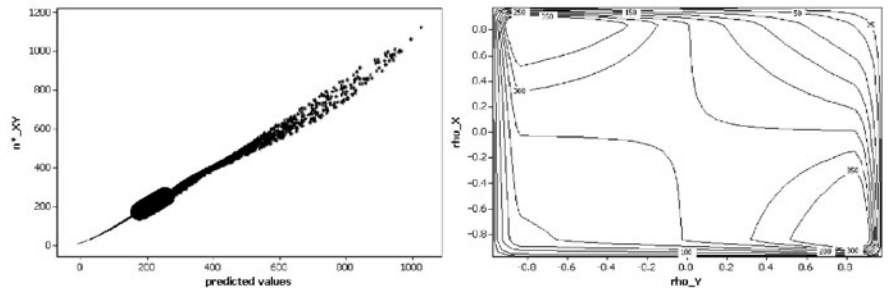
Fig. 5.5 Left (a): the approximate bivariate relationship between \hat{n}_{XY}^* and \hat{n}_X^* and \hat{n}_Y^* for \rho_X > 0 & \rho_Y > 0 denoted by dots (.), \rho_X < 0 & \rho_Y < 0 , denoted by solid circles (●), and mixtures, denoted by asterisks (*). Right (b): a contour map of the joint relationship between \hat{n}_{XY}^* and \rho_X and \rho_Y
