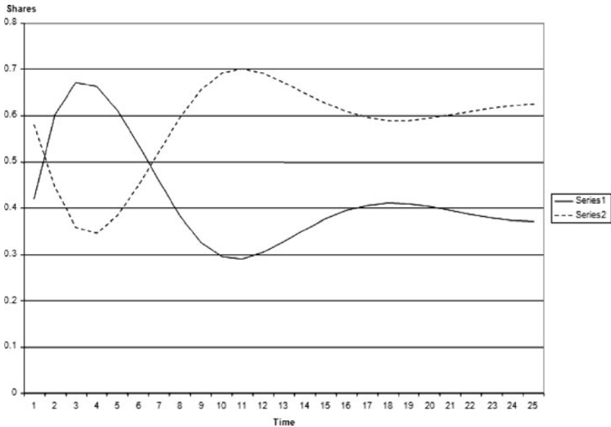
Fig. 15.3 First region simulatioins results graphed
