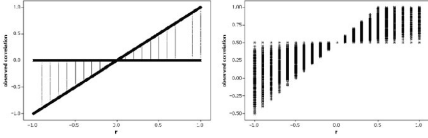
Fig. 5.6 Relationships between the spatially adjusted correlation coefficient, r , and the spatially unadjusted correlation coefficient. Left (a) : the case of no common eigenvectors in the spatial filters. Right (b) : the case of common eigenvectors in the spatial filter that account for 50% of the variance
