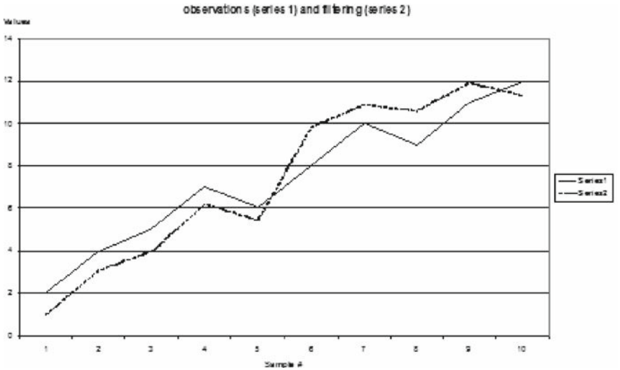
Fig. 17.1 The spatial series y and y^*
