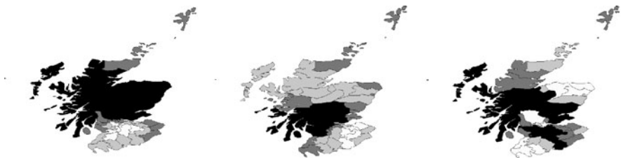
Fig. 7.4 Spatial filter map patterns (i.e., eigenvectors E_1 , E_2 and E_9 ) common to Y , \text{LN}(X_1 + 1.2) , and \text{LN}(X_2/\text{area} - 22.2)
