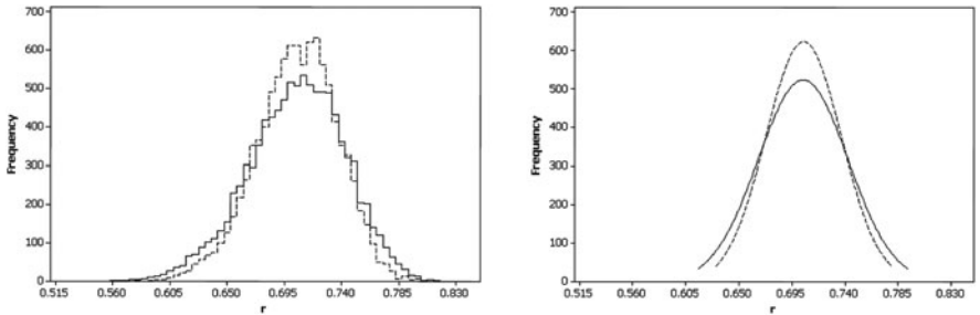
Fig. 5.3 Computer-generated sampling distributions of the correlation coefficient, r . Broken lines (---) denote r computed with spatially unautocorrelated data values; solid lines (—) denote r computed with spatially autocorrelated data values. Left (a): histograms. Right (b): normal curve approximations to the histograms
