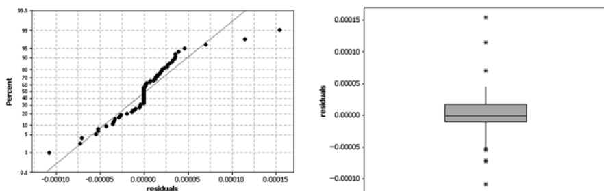
Fig. 6.3 Graphical diagnostics of residuals for the GLMM estimated with SAS. Left (a): normal quantile plot. Right (b): boxplot
