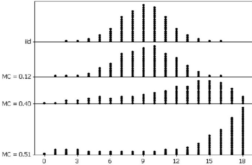
Fig. 4.21 Dot plot versions of histograms for the MCMC auto-binomial simulated data. Top (a): iid. 2nd from top (b): weak positive SA. 2nd from bottom (c): low moderate positive SA. Bottom (d): moderate positive SA
