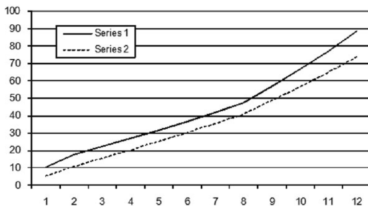
Fig. 13.5 Dutch model, binary case
