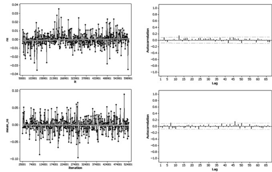
Fig. 6.4 A average random effects term example MCMC chain from a WinBUGS run in which the random effects intercept was spatially structured. Top left (a): a time series plot from an ICAR model with a trend line ( gray ) superimposed. Top right (b): a correlogram from an ICAR model with a 95% confidence interval ( gray ) superimposed. Bottom left (c): a time series plot from a SF model with a trend line ( gray ) superimposed. Bottom right (d): a correlogram from a SF model with a 95% confidence interval ( gray ) superimposed.
