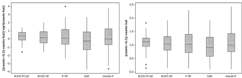
Fig. 7.5 Boxplots of deviations produced by the various model specifications. Auto-P: Winsorized auto-Poisson; BUGS-PCAR: GeoBUGS proper CAR; BUGS-SF: BUGS spatial filter; P-SF: Poisson spatial filter; and, SAR: simultaneous autoregressive. Left (a) standardized residual counts. Right (b) : ratio of observed to expected SMRs
