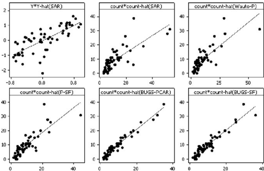
Fig. 7.8 Scatterplots of model predicted versus observed counts. Top left (a): SAR normal approximation transformed. Top center (b): SAR back-transformed normal approximation. Top right (c): Winsorized auto-Poisson counts. Bottom left (d): Poisson spatial filter. Bottom center (e): Geo-BUGS proper CAR HGLM. Bottom right (f): BUGS spatial filter HGLM
