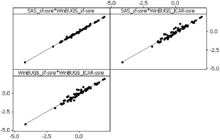
Fig. 6.6 Scatterplot of the SAS and mean WinBUGS estimated spatially structured random effects term. Top left (a) : the SAS versus WinBUGS results based upon SF models. Top right (b) : the SAS SF model results versus the WinBUGS ICAR model results. Bottom left (c) : the WinBUGS SF versus ICAR model results
