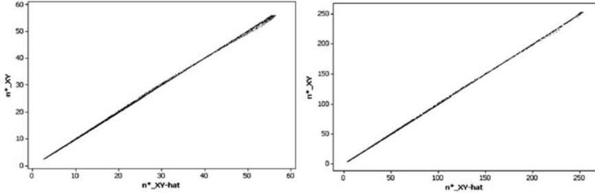
Fig. 5.2 Simulation-based relationships between a composite of individual univariate effective sample sizes and their corresponding bivariate effective sample size. Left (a) : Scotland results based upon a Bessel function and Eq. (5.4a). Right (b) : Murray smelter site results based upon a Bessel function and Eq. (5.4b)
