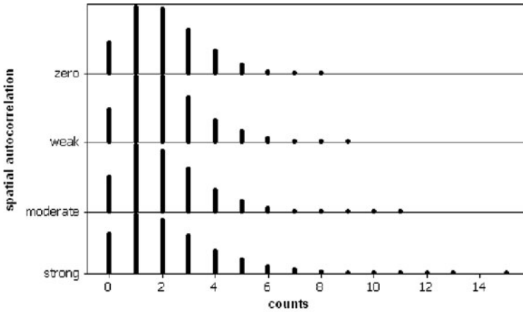
Fig. 7.3 Dotplot of Poisson counts with increasing levels of positive spatial autocorrelation
