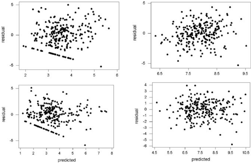
Fig. 8.5 Conventional homogeneity of variance scatter plots. Left (a): top, for spatial SAR model describing As; bottom, for spatial filter model describing As. Right (a): top, for spatial SAR model describing Pb; bottom, for spatial filter model describing Pb
