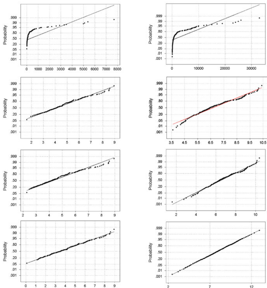
Fig. 8.2 Evolution of the pollutant data transformation quantile plots. Left (a) : from top to bottom, raw As values, logarithmic As values, Eq. (8.1) As values, and Eq. (8.2) As values. Right (b) : from top to bottom, raw Pb values, logarithmic Pb values, Eq. (8.1) Pb values, and Eq. (8.2) Pb values
