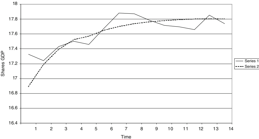
Fig. 11.4 GDP time-series plot: eastern Netherlands
