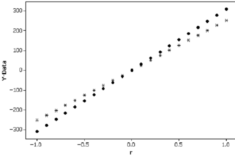
Fig. 5.4 Average cross-product terms for simulated data based upon the Murray smelter site. Asterisks (*) denote spatially autocorrelated data; solid circles (●) denote spatially unautocorrelated data
